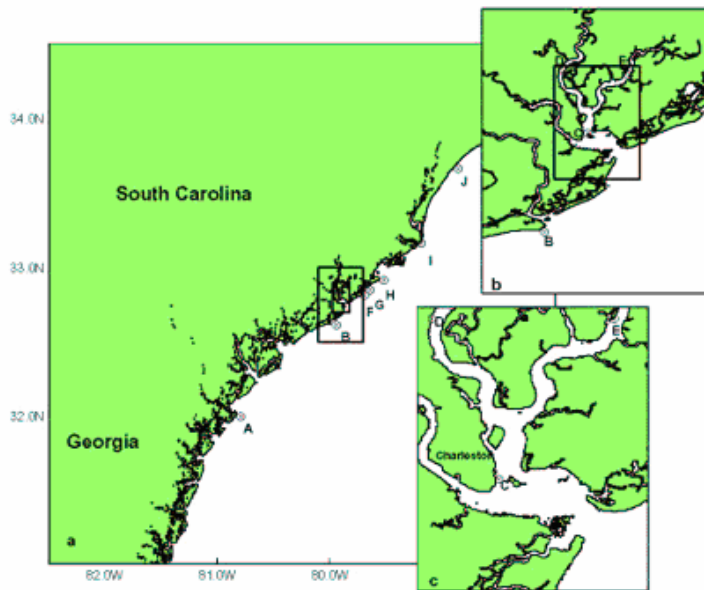
Figure 3. Triple nesting for Charleston region.
